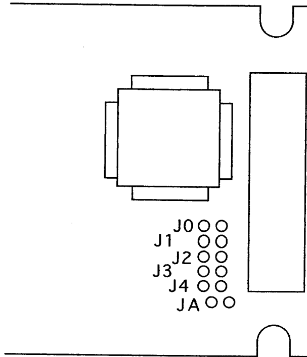
PCB PARTS SIDE
